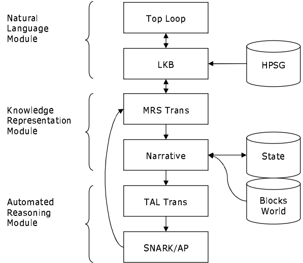
Figure 2: An overview of the NL1 architecture.
